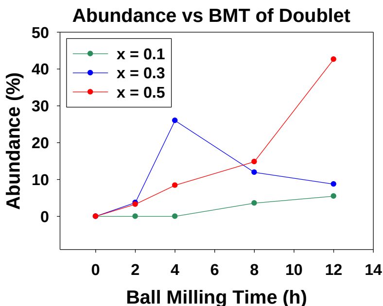
Figure 4: Abundance of the quadrupole split doublet on the ball milling time showing the production of terbium iron perovskite.
