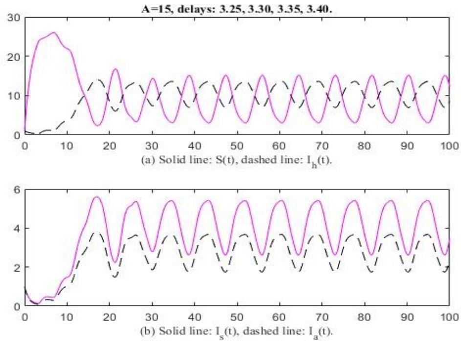
Fig. 3: Oscillation of the solutions, A=15 , delays: 3.25, 3.30, 3.35, 3.40.
