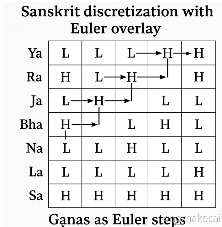
Figure 4: Eulerian steps mapped onto a Chandas grid, illustrating local-to-global iteration across metrical traditions. Diagram generated with Grok xAI and validated by the authors.
