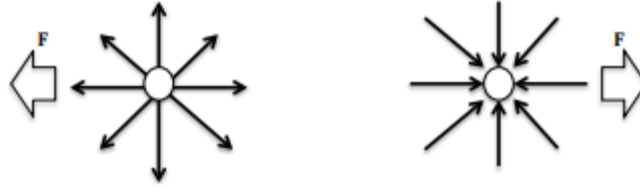
Fig. 4.5: A positive and a negative g-charges repel each other
