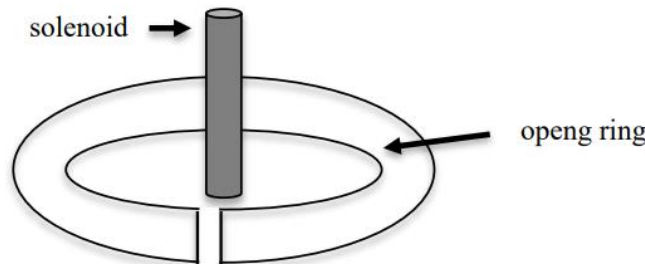
Fig. 5.3 Setup: Spin-Potential-Coupling-Induced Force: open ring and solenoid
