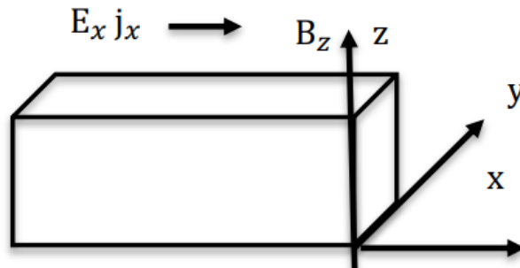
Fig. 5.1 Setup: Extended-Hall Effect/Topological Insulator
