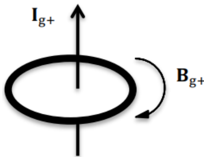
Figure. 4.7: “The left-hand rule” for gravito-magnetic field \mathbf{B}_{g+}
