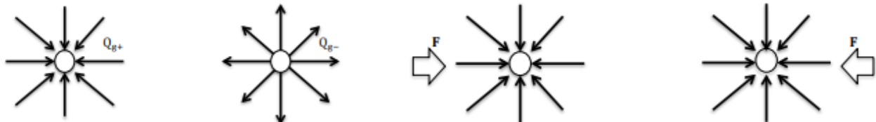
Fig. 4.1. Field line of Q_{g+} , Fig. 4.2. Field line of Q_{g-} Fig. 4.3: two positive g-charges are attractive to each other
