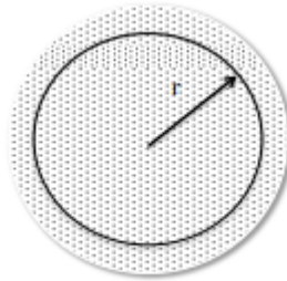
Fig. 4.6: Accelerating Expansion of Universe
