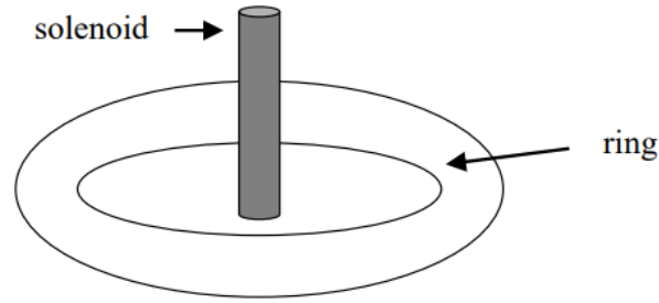
Fig. 5.2 Setup: Spin-Potential-Coupling-Induced Force: ring and solenoid
