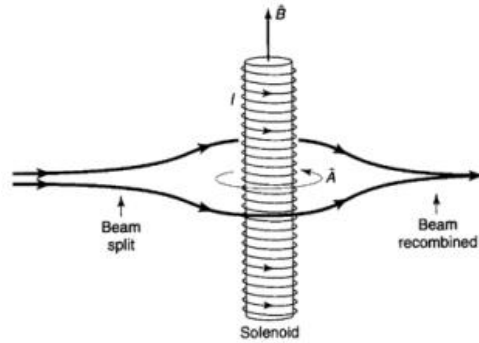
Fig. 5.4 Setup: Spin-Potential-Coupling Force Contributing to Aharonov-Bohm Effect
