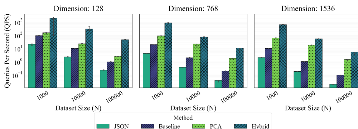
Figure 4: Search Time Comparison (Log Scale). JSON incurs the highest latency, while Hybrid Search minimises retrieval time
