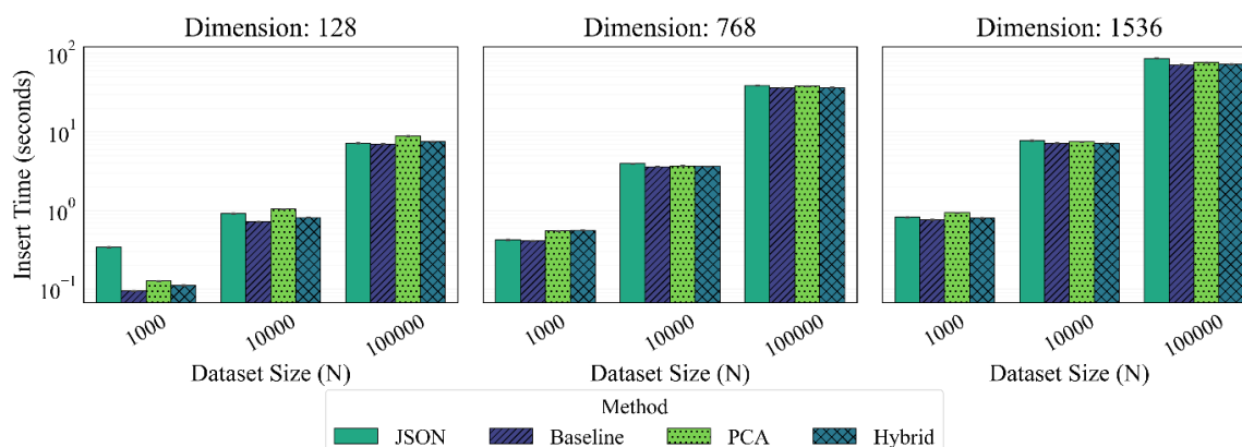
Figure 5: Insertion Time Comparison (Log Scale). Binary VECTOR storage offers slight improvements over JSON text storage.
