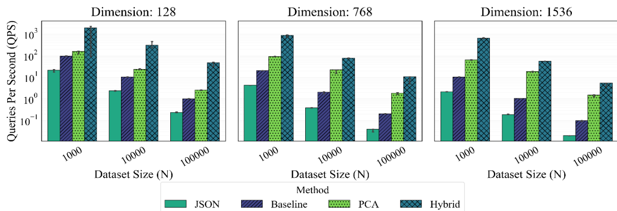
Figure 2: Throughput (QPS) Comparison. Hybrid Search consistently outperforms other methods.
