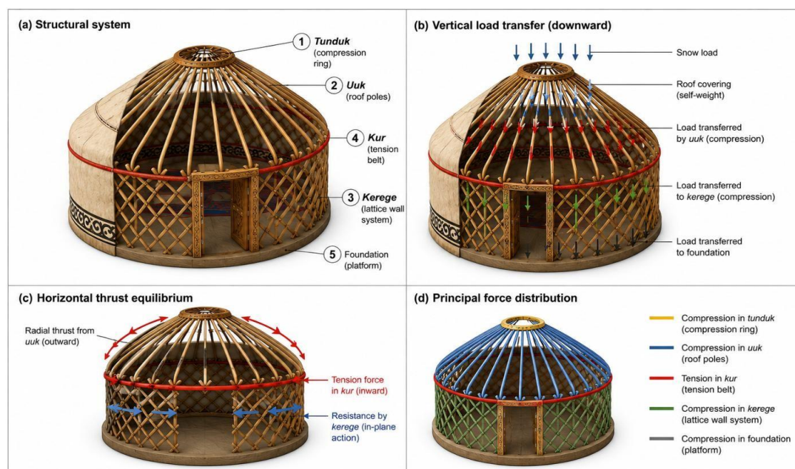
Figure 2: Load transfer mechanism in the Kyrgyz yurt: (a) structural system; (b) vertical load path; (c) equilibrium of horizontal thrust forces through the tension belt (kur); (d) principal force distribution within the structural system.
