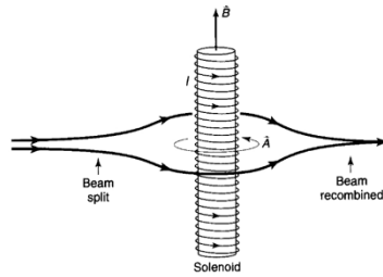
Figure 3.1: Setup: Spin-Potential-Coupling Force Contributing to Aharonov-Bohm Effect
