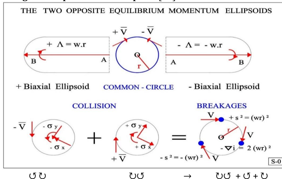
Figure 16: The work W , of Two-Quaternion-monads \bar{z} = (s + \bar{v}.V_i) \equiv \bar{AB} \equiv \bar{w} is the Action of any two Tangential & Opposite Equilibrium-Dipole [\oplus \leftrightarrow \ominus] with v = \bar{w}.r .
