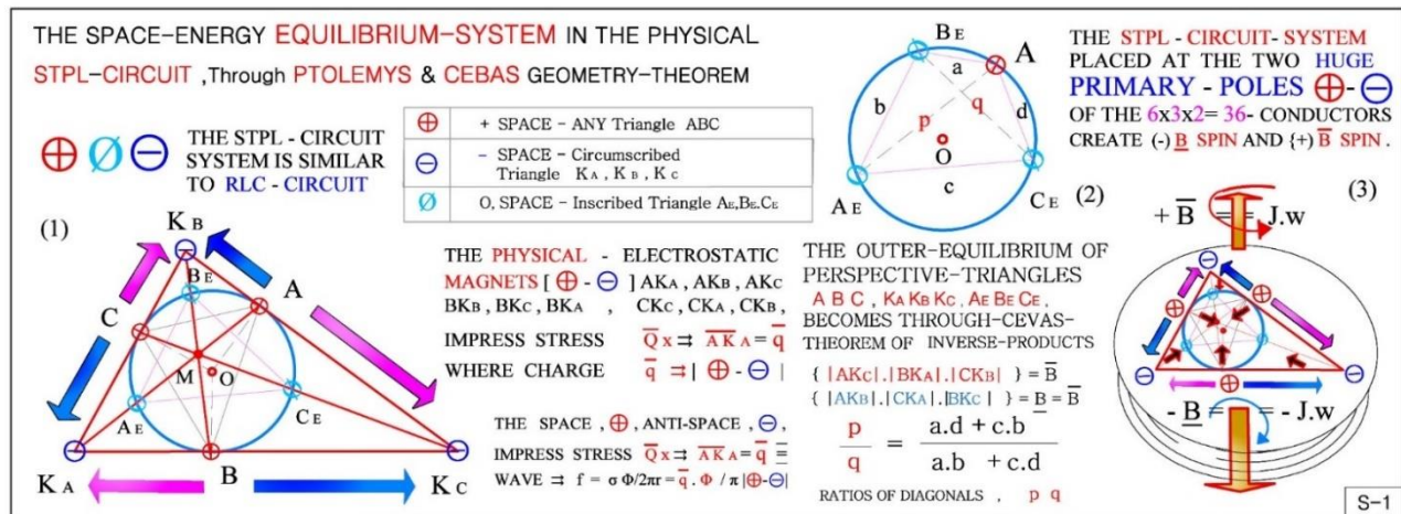
Figure 24: The Stability of \rightarrow \{\oplus - \text{Space } [A B C]\} , \{\ominus - \text{Anti-Space } [K_A K_B K_C]\} , of The Sub-Space [A_E, B_E, C_E] , and Neutral-Space \{\{\oplus \leftrightarrow \ominus\} \equiv ds \equiv \{\oplus \leftarrow ds \rightarrow \ominus\}\} .
