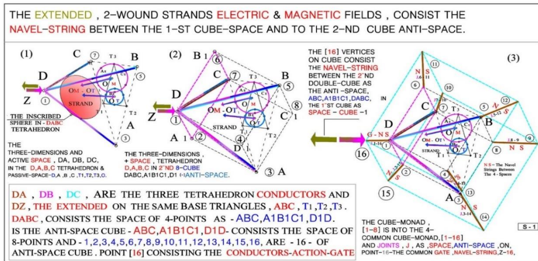
Figure 29: The Electric - Magnetic Field of 3, Conductors Results on 2 -Anti-Parallel-Strands. The Stability of \rightarrow \{\oplus 4\text{-Space } [D A B C]\} Regular - Tetrahedron , IN \{\ominus 8\text{-Anti-Space Cube, } [DA_1B D_1, C C_1AB_1]\} , and The \rightarrow \{\oplus 8\text{-Space } [DA_1BD_1, CC_1AB_1]\} Cube , INTO The \{\ominus 16\text{-Anti-Space } [1,2,3,4,5, 6, 7, 8 - 9,10,11, 12, 13,14, 15, 16]\} Sphere Cube Vertices . Point [16 \equiv |z|Z| ] consists the Navel-String Gate in \{Z-(\Delta D, ABC), \Delta[T1 T2 T3]\} Stationary Bases. Stability Analysis in [88]
