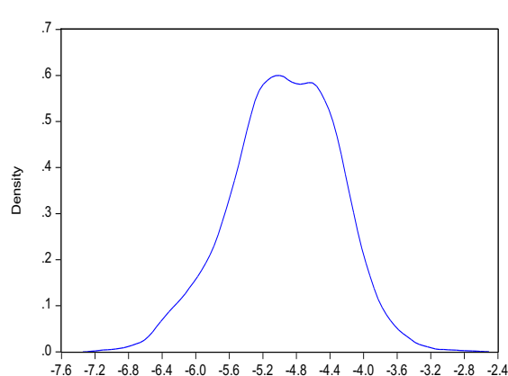
Fig. 12. Kernel density of model AA
